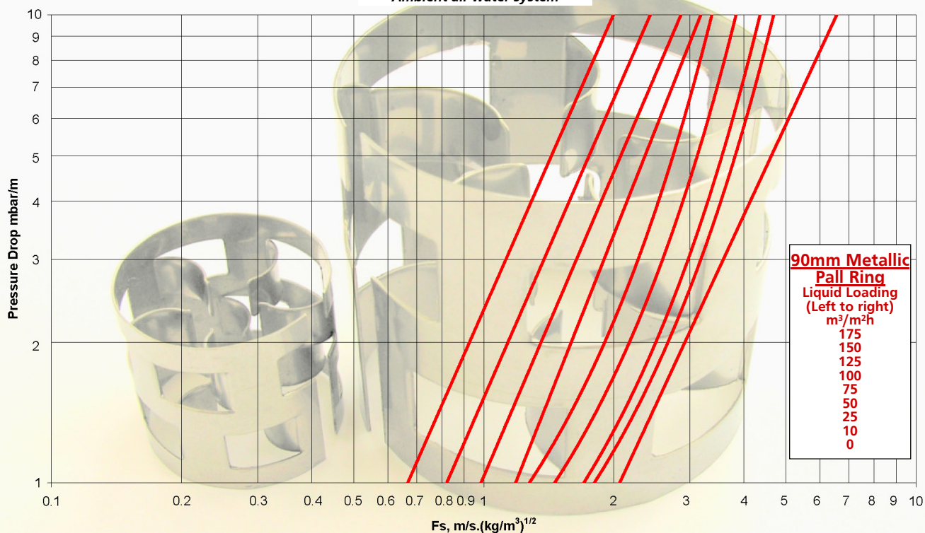
90mm Metallic Pall Ring Ambient air-water system
