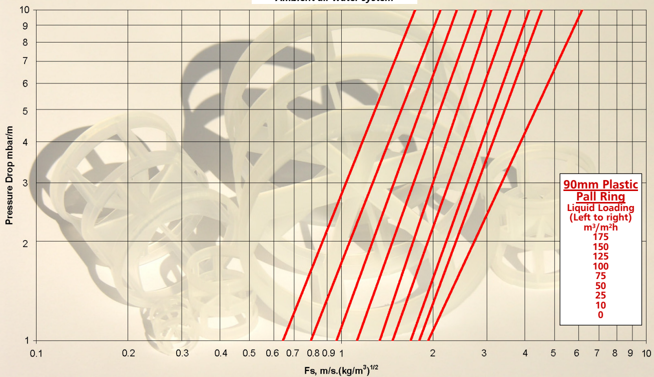
90mm Plastic Pall Ring Ambient air-water system
