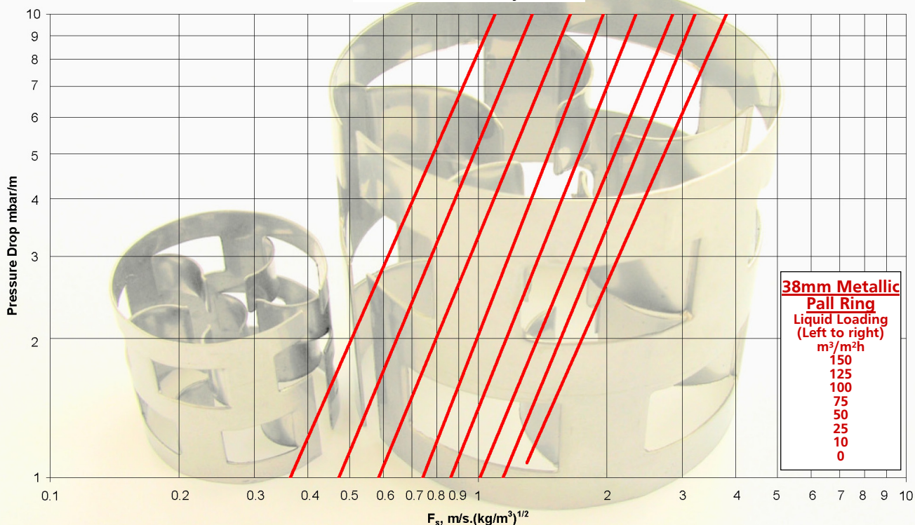
38mm Metallic Pall Ring Ambient air-water system
