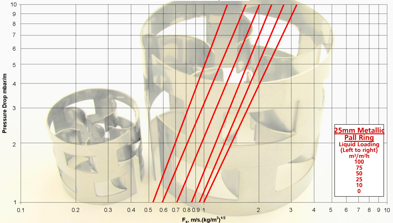
25mm Metallic Pall Ring Ambient air-water system
