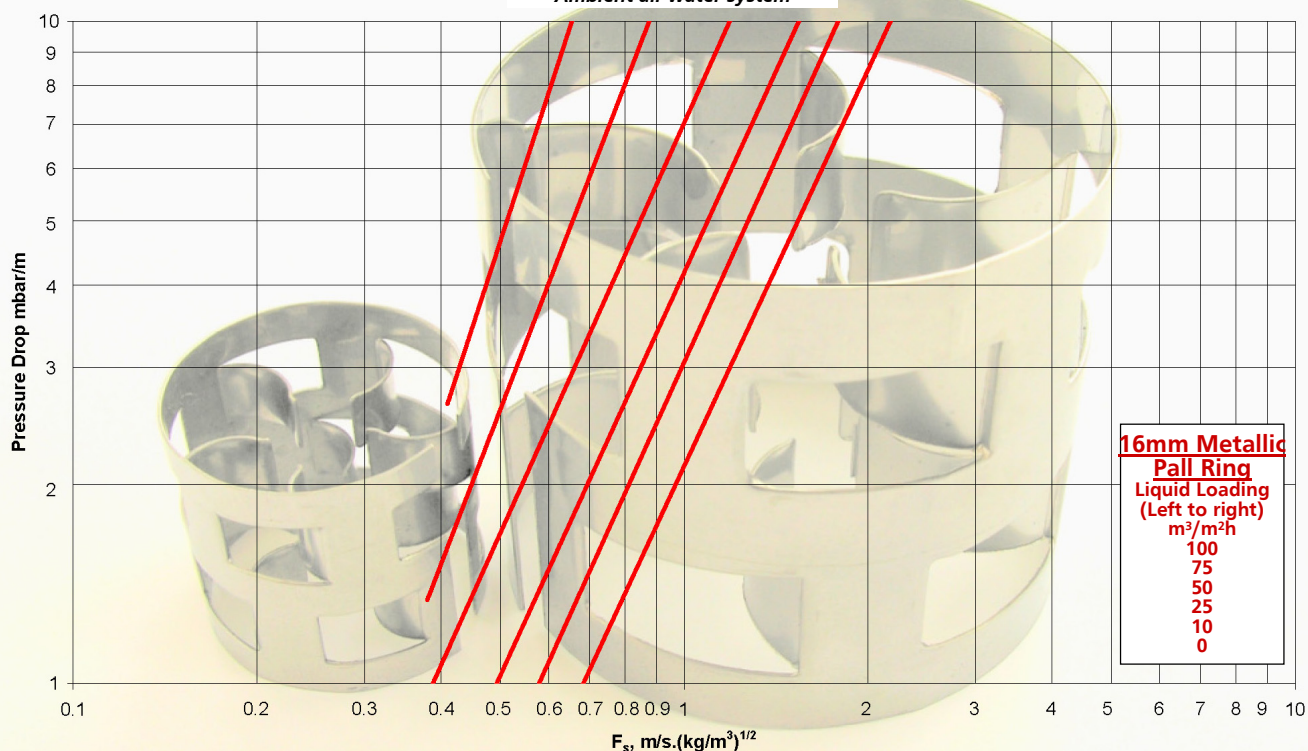
16mm Metallic Pall Ring Ambient air-water system
